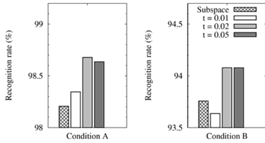
Fig. 7 Recognition rates under conditions A and B.
