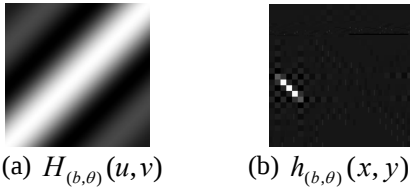
Fig. 2. Example of motion-blur PSF ( b = 5 , \theta = \pi/4 ).
