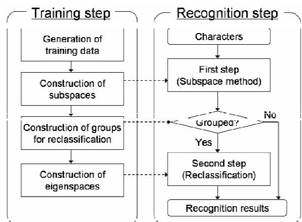
Fig. 1. Flow of proposed method.
