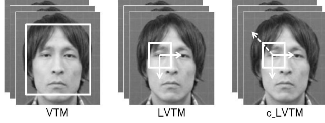
Fig. 6. The difference in how the image patterns are selected for the transition model computation between VTM, LVTM and the proposed c-LVTM method.
